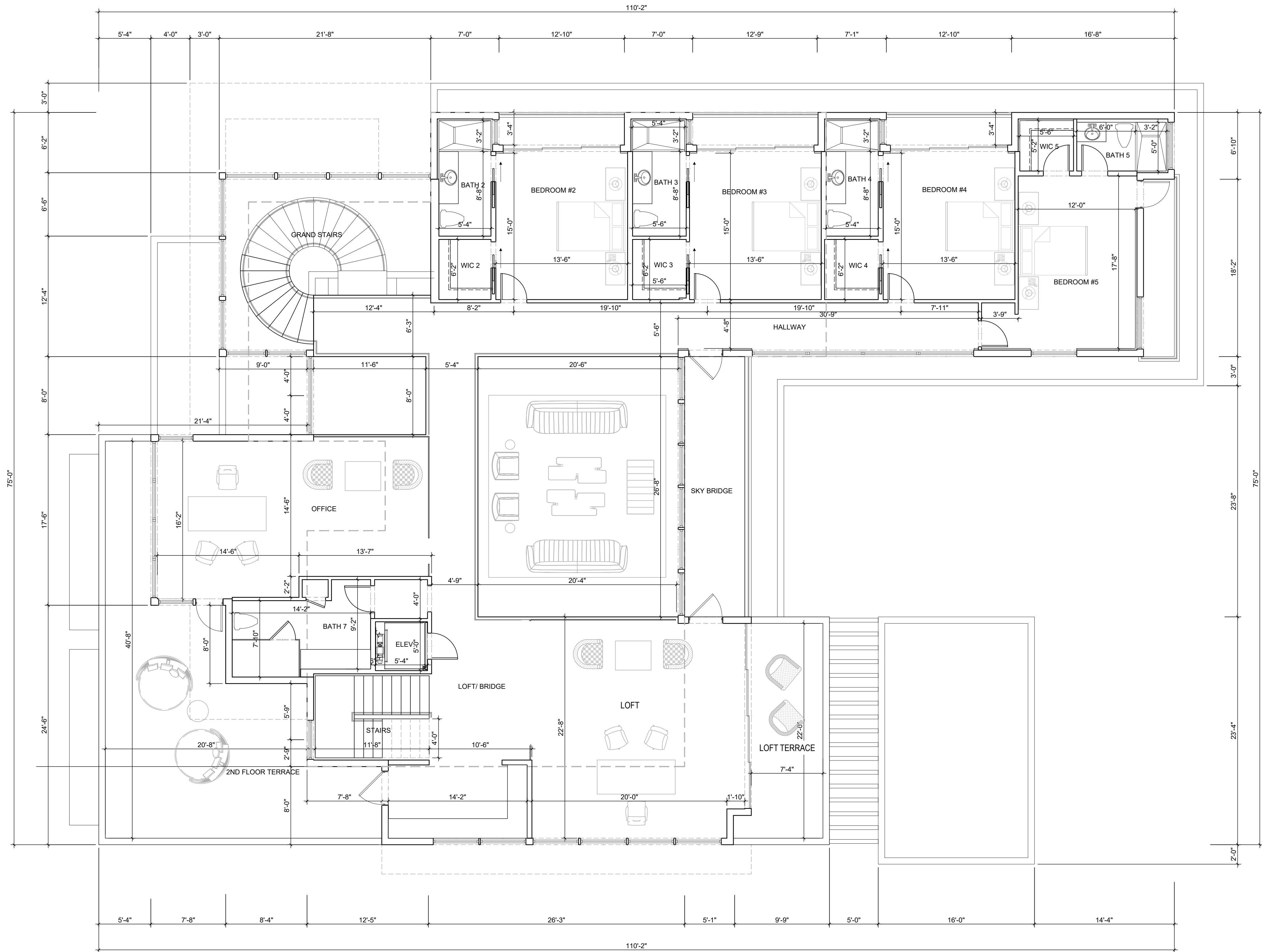
2ND. DIMENSION PLAN SCALE 3/16" = 1'-0"
